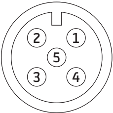
24VDC M-12 Power Connector (MALE)
