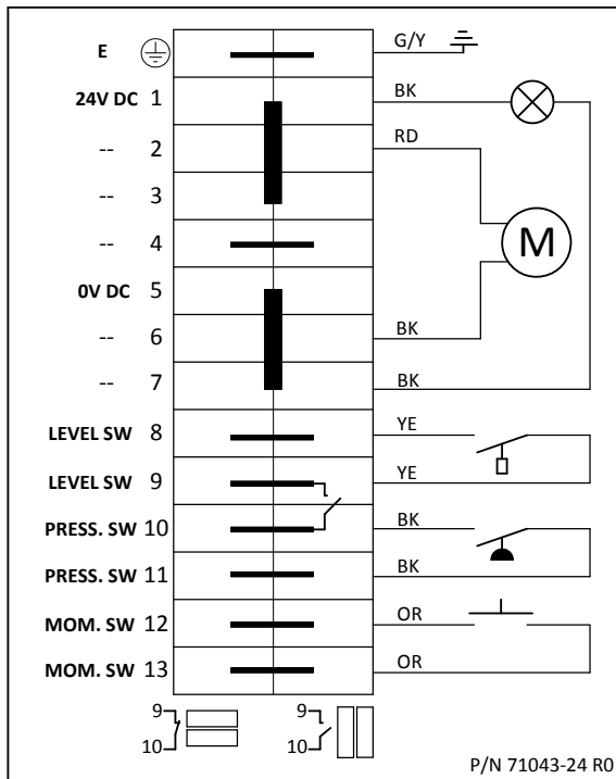
Terminal Strip
