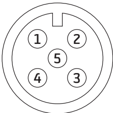
24VDC M-12 Signal Connector(FEMALE)
