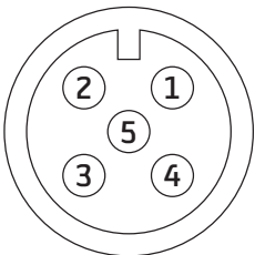
115/230VAC M-12 Signal Connector(MALE)
