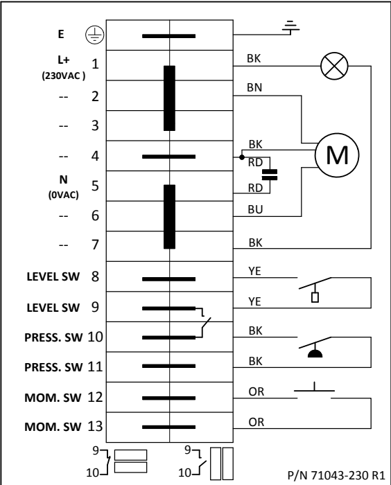
Terminal Strip
