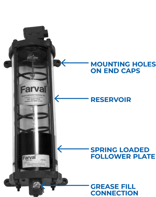
Grease Reservoir T30P5AC (Shown without pump attached)
